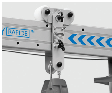
CARRELLO CHIUSO PGTXR00500 - WLL 500 kg - 1 operatore PGTXR01000 - WLL 1000 kg - 1 operatore
