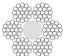
6x19N+PP 114 fili/wires
