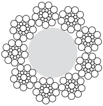
8(9+9+1)S+FC 152 fili/wires
