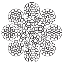
8xK31WS+PWRC 359 fili/wires
