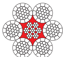
6xK31WS+EPIWRC 235 fili/wires
